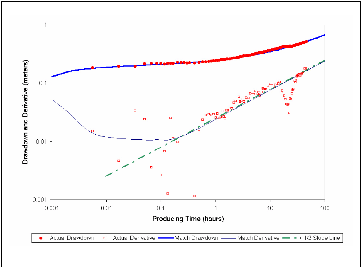
Figure 4.1-14 Log-Log Diagnostic Plot for NC-EWDP-1S Showing +1/2 Slope in Derivative Characteristic of Parallel Boundaries
