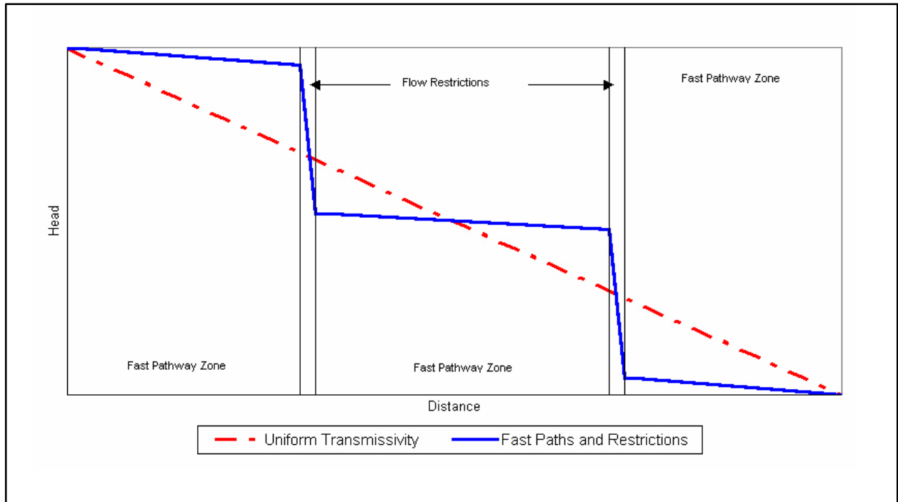
Figure 4.1-11 Conceptual Head Changes along a Flow Pathline
