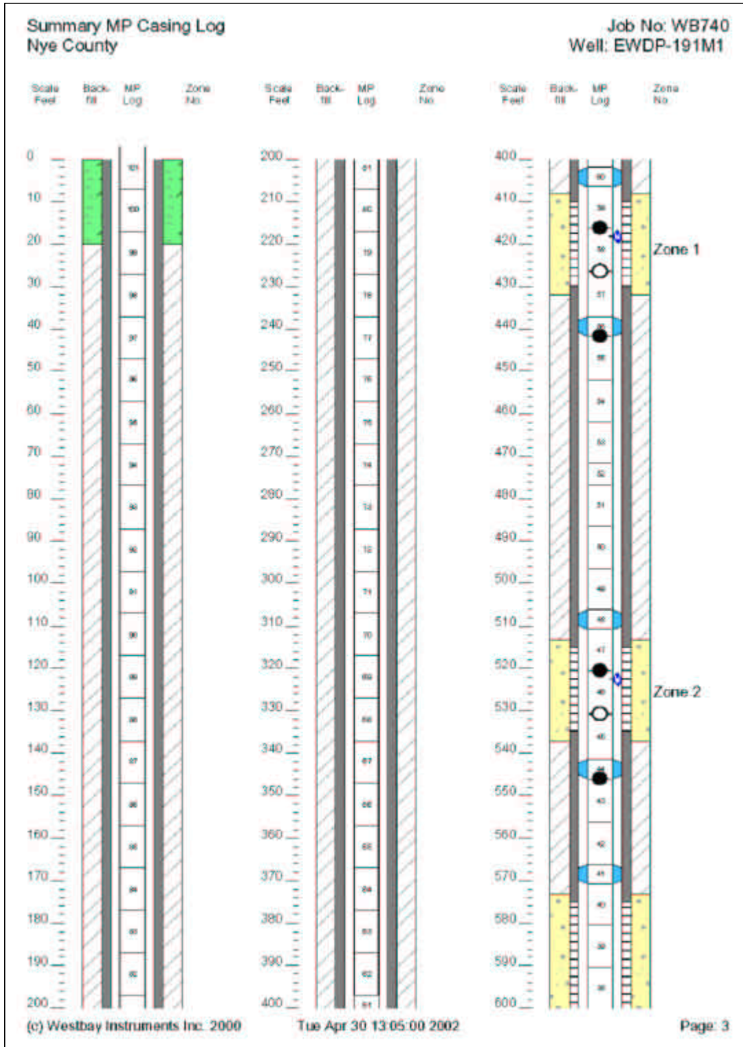
Figure C2 Westbay® Summary Casing Log for Well NC-EWDP-191M1 (3 of 4)
