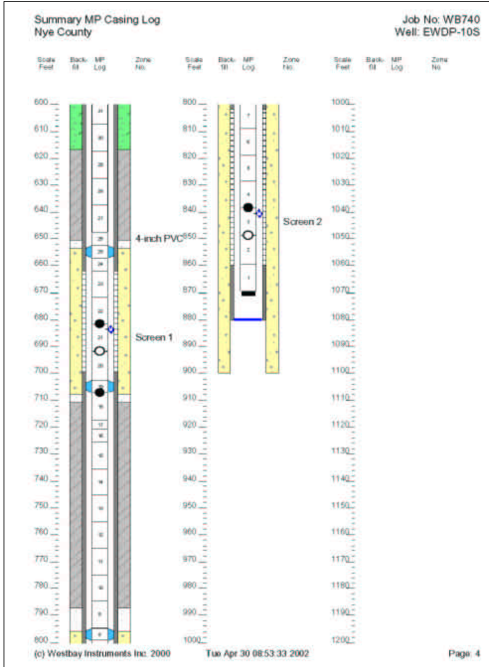
Figure C1 Westbay® Summary Casing Log for Well NC-EWDP-10S (4 of 4)
