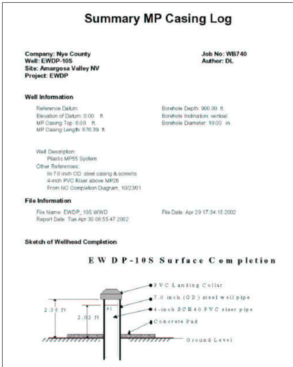
Figure C1 Westbay® Summary Casing Log for Well NC-EWDP-10S (1 of 4)
