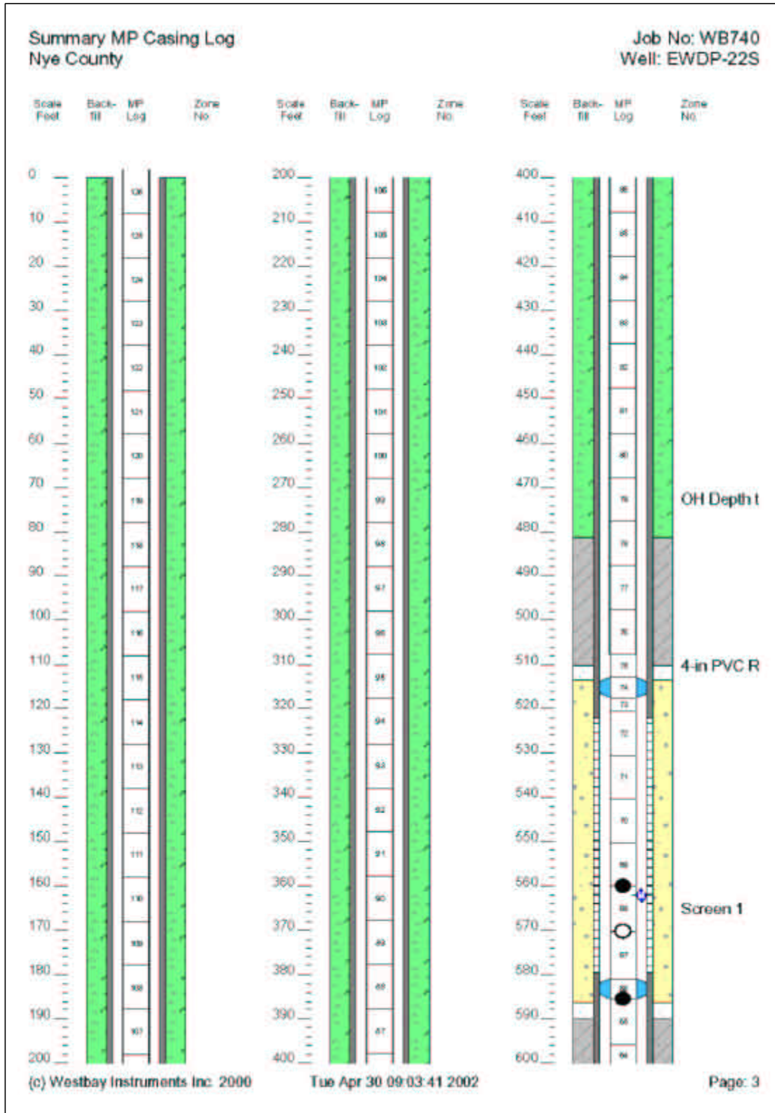
Figure C3 Westbay® Summary Casing Log for Well NC-EWDP-22S (3 of 4)
