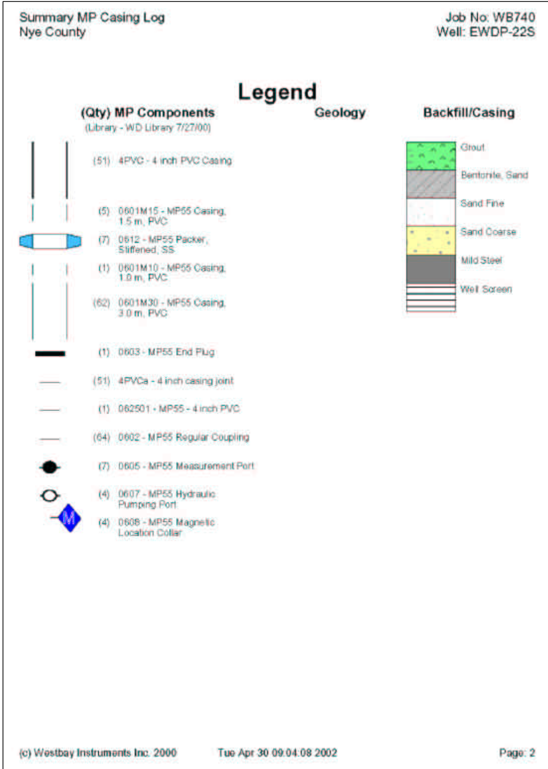
Figure C3 Westbay® Summary Casing Log for Well NC-EWDP-22S (2 of 4)
