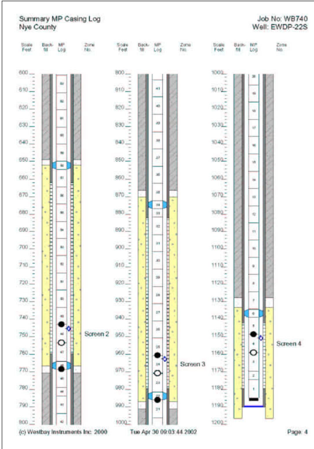
Figure C3 Westbay® Summary Casing Log for Well NC-EWDP-22S (4 of 4)
