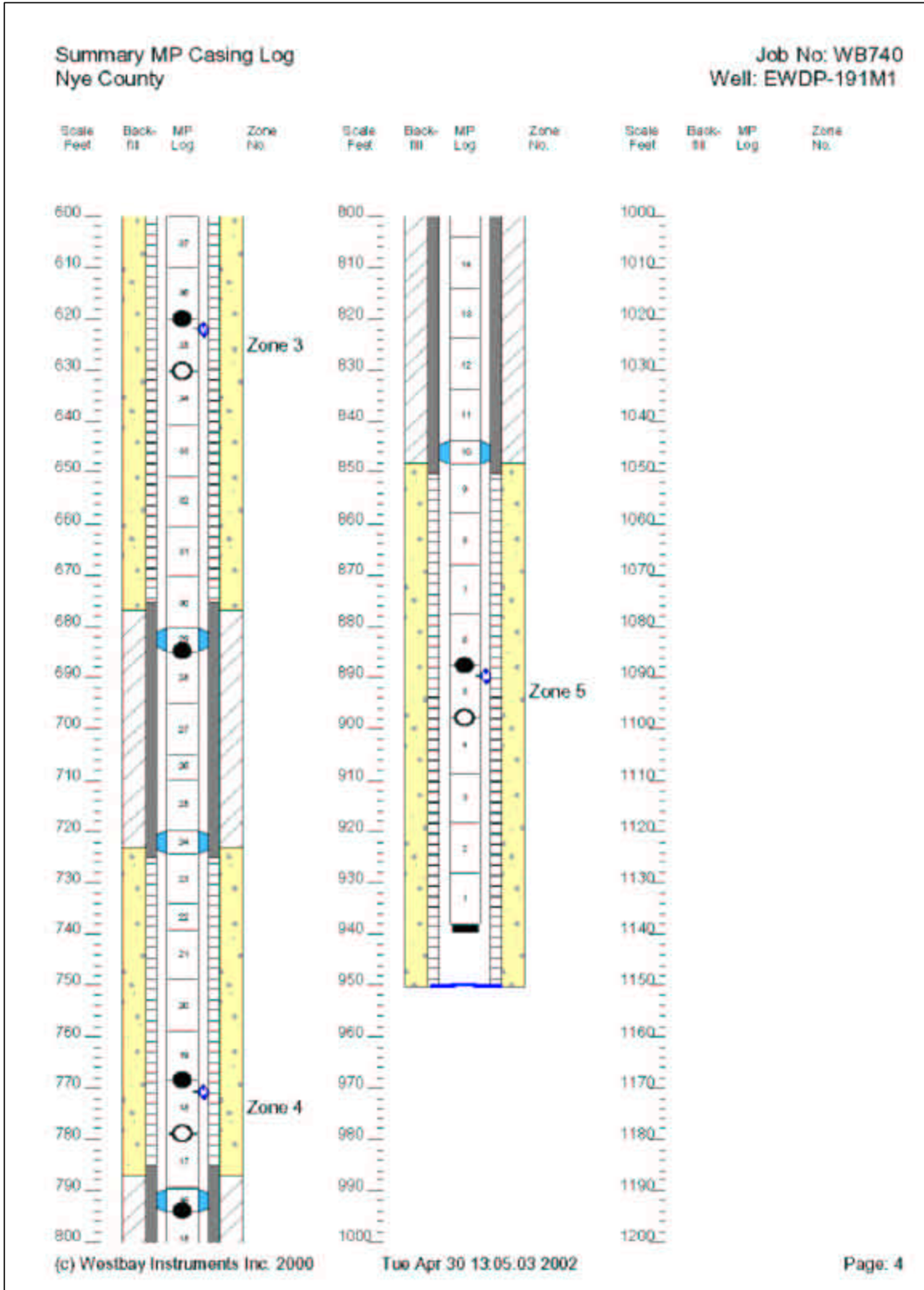
Figure C2 Westbay® Summary Casing Log for Well NC-EWDP-191M1 (4 of 4)
