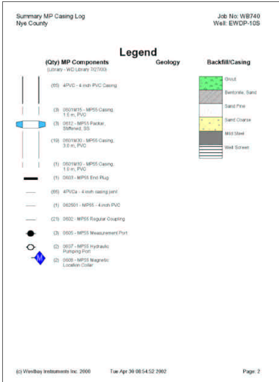
Figure C1 Westbay® Summary Casing Log for Well NC-EWDP-10S (2 of 4)
