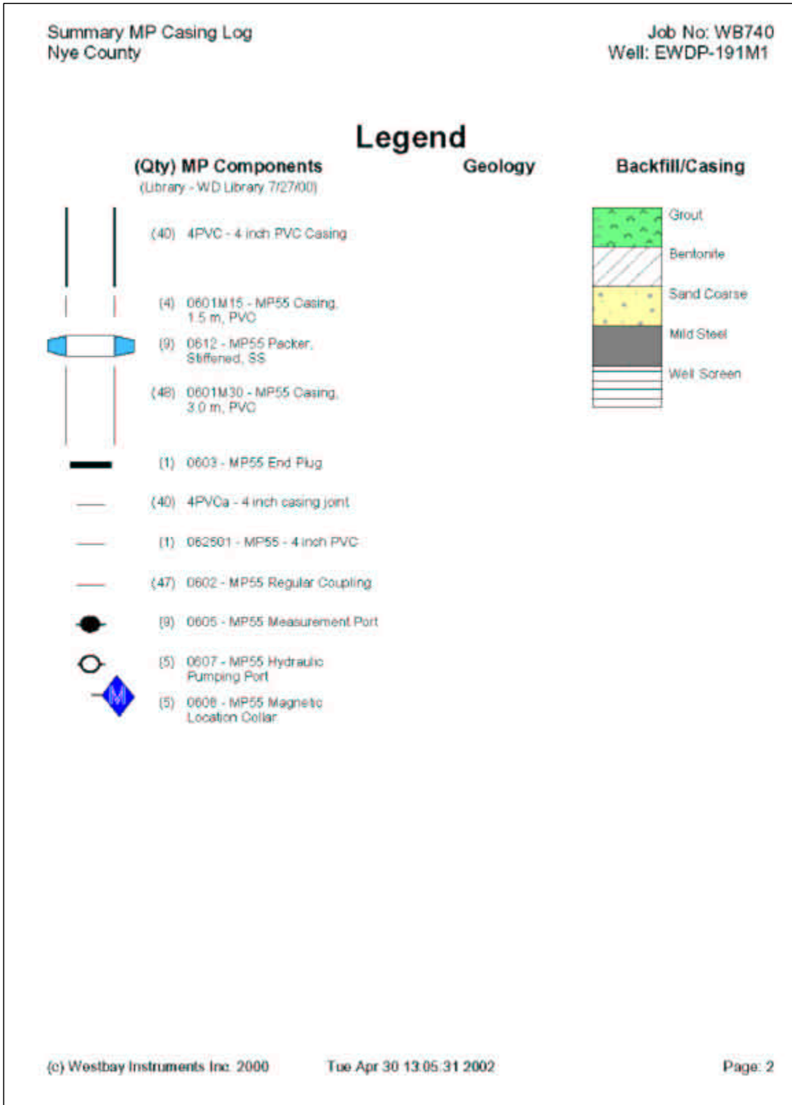
Figure C2 Westbay® Summary Casing Log for Well NC-EWDP-191M1 (2 of 4)
