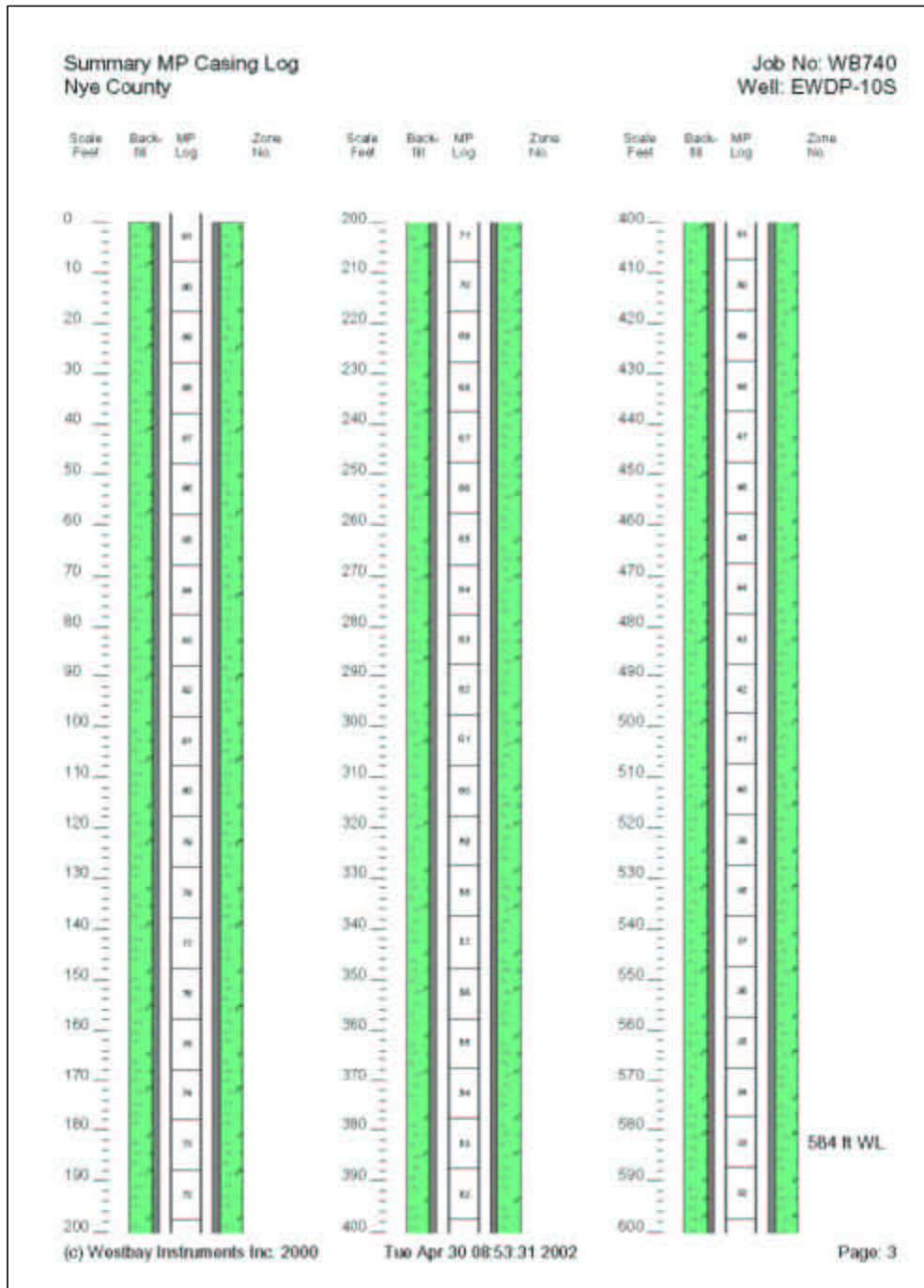
Figure C1 Westbay® Summary Casing Log for Well NC-EWDP-10S (3 of 4)
