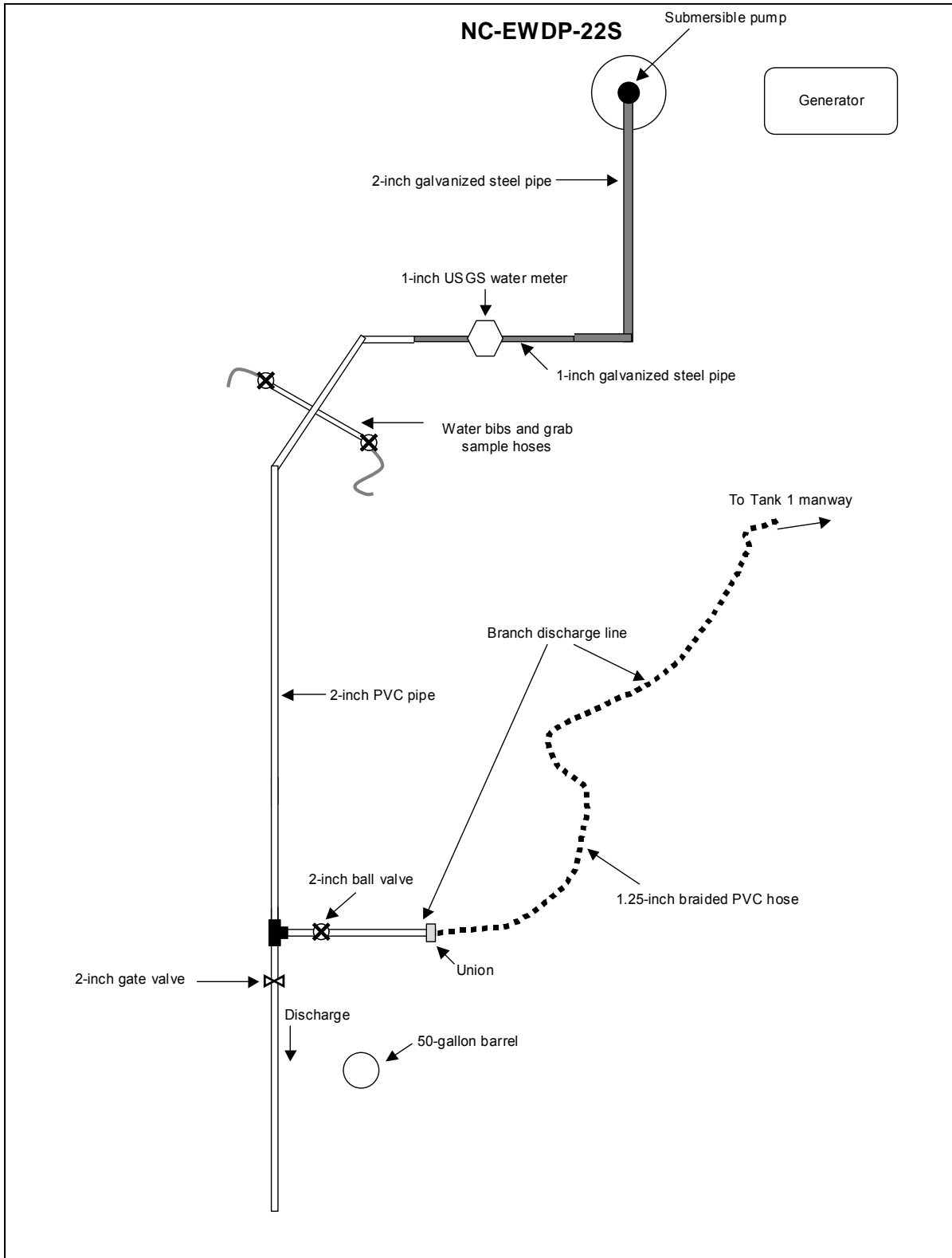
Figure 4 Piping Schematic for Rinsing and Filling of Tank 1 with Water
